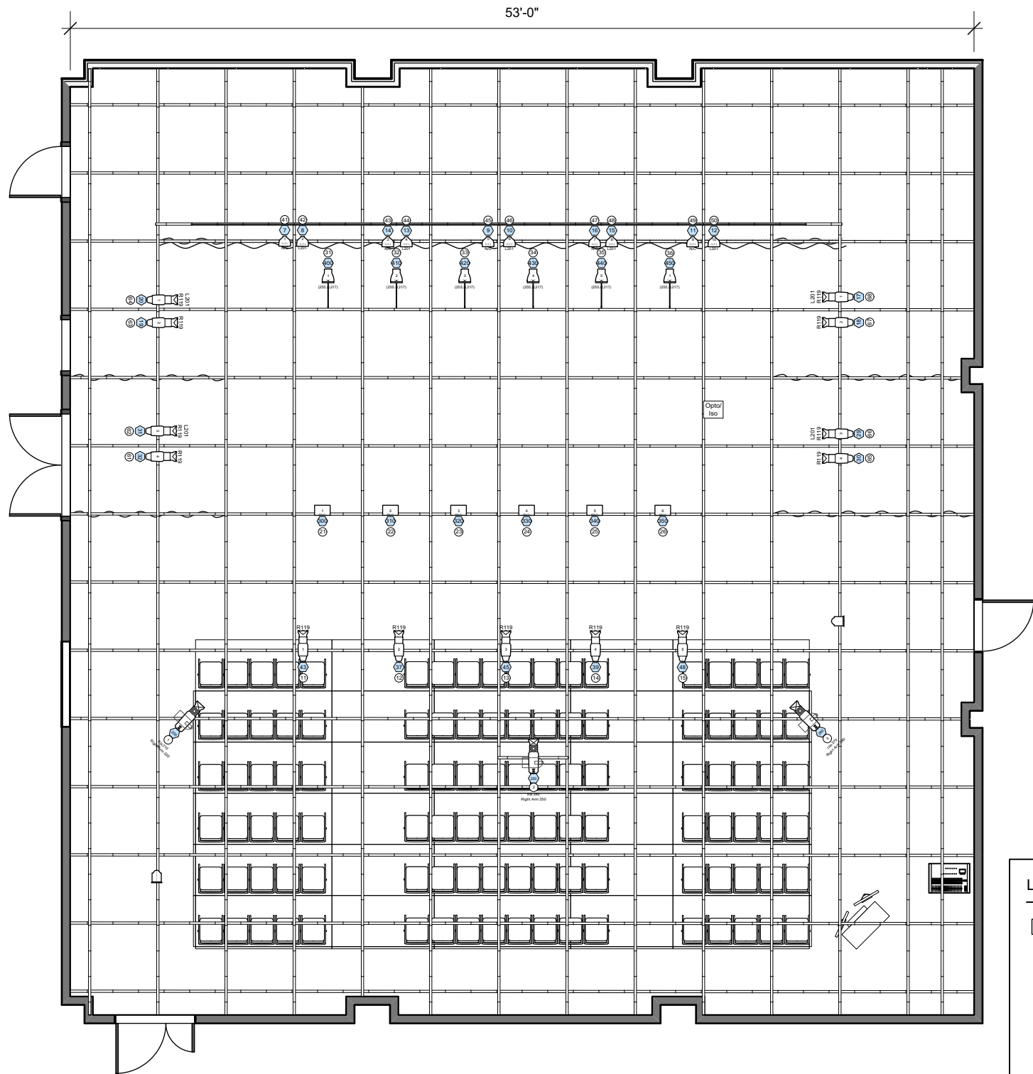
1 OBT Rep Plot Scale: 1/8" = 1'-0"
